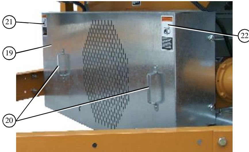
Bottom auger and metering roll drive guard.
